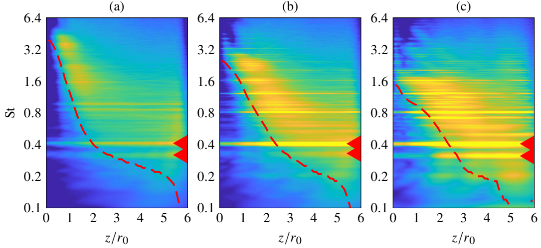
Figure 11: PSD of the radial velocity fluctuations of aerodynamic nature normalized by u_j , at r = r_0 , for the jets at M = 0.9 with (a) \delta_{BL} = 0.05r_0 , (b) \delta_{BL} = 0.1r_0 and (c) \delta_{BL} = 0.2r_0 , for n_\theta = 0 ; \blacktriangle Strouhal numbers of the tones A_1 and A_2 ; --- most unstable Strouhal numbers for n_\theta = 0 according to LSA. The color scales range logarithmically from (D/u_j) \times 10^{-6} to (2D/u_j) \times 10^{-2} , from blue to yellow.
