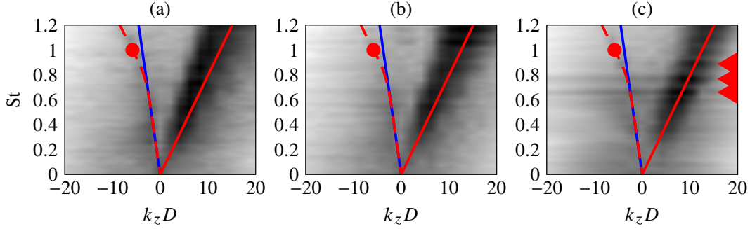
Figure 21: Frequency-wavenumber spectra of the pressure fluctuations computed for n_\theta = 0 at r = r_0 for the jets at M = 0.6 with (a) \delta_{BL} = 0.05r_0 , (b) \delta_{BL} = 0.1r_0 and (c) \delta_{BL} = 0.2r_0 ; — \omega/k_z = 0.5 \times u_j and — \omega/k_z = -c_0 ; - - - dispersion curve of the GJW for a vortex-sheet model; ● first least-dispersed GJW; ◀ Strouhal numbers of the peaks in the near-nozzle spectra for \delta_{BL} = 0.2r_0 . The color scale ranges logarithmically from the minimal to the maximal values from white blue to black.
