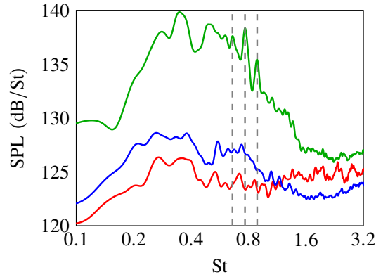
Figure 17: Sound pressure levels at z = 0 and r = 1.5r_0 for the jets at M = 0.6 with \delta_{BL} = 0.05r_0 , \delta_{BL} = 0.1r_0 and \delta_{BL} = 0.2r_0 ; - - - Strouhal numbers of the narrow peaks for \delta_{BL} = 0.2r_0 .
