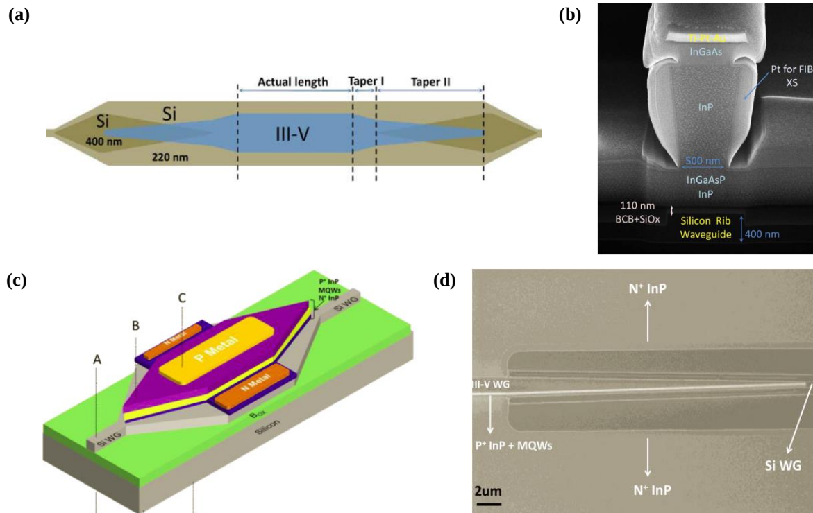
Figure IV-1: (a) Schematic view of a inverted double-taper architecture, and (b) scanning electron microscope image of its III-V tip [60]. (c) Schematic view of a same direction double-taper architecture and (d) scanning electron microscope image of its III-V tip [153].
