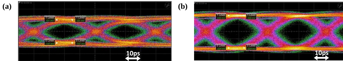
Figure II-44: Eye diagrams at 25\text{Gb/s} of the electrical signal send on the RF probes: (a) without de-emphasis, (b) with de-emphasis.
