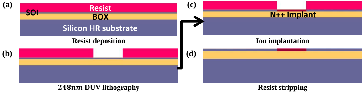
Figure II-23: Implantation steps for Si-doping
