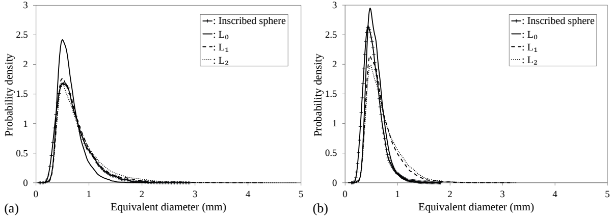
Figure 8: Probability density functions for the equivalent pore diameter resulting from different definitions and corresponding to the overlapping inscribed void spheres technique; (a): GGL, (b): GGD
