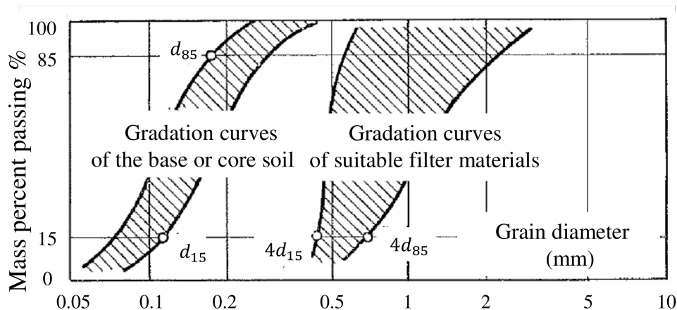
Fig. II.4. Filter and drainage criteria (Terzaghi et al., 1996)
