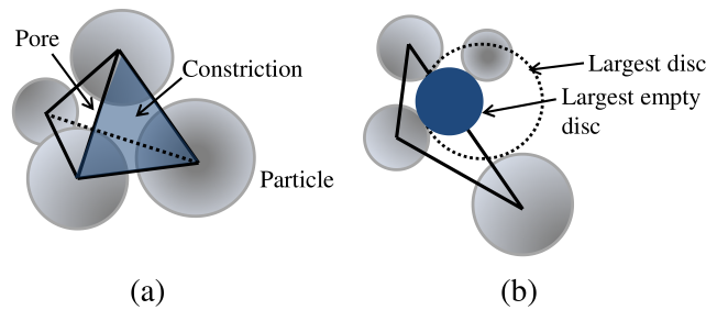
Figure 1: (a) : Tetrahedron built from the centers of four neighboring spheres; (b) : Definition of a constriction: the largest disc included in the void space for a given face
