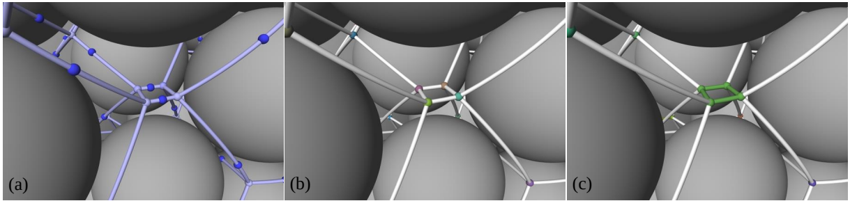
Figure 6: Detail of spheres and Voronoï graph extracted from the GGD sample; (a): Bright spheres at crossings indicate pore centers, darker spheres indicate constrictions; (b): Unmerged pore centers are randomly colored by their label ID; (c): Merged pore centers and their connection paths and constrictions will be labeled as belonging together ( t = 1\% ) (color figure online)
