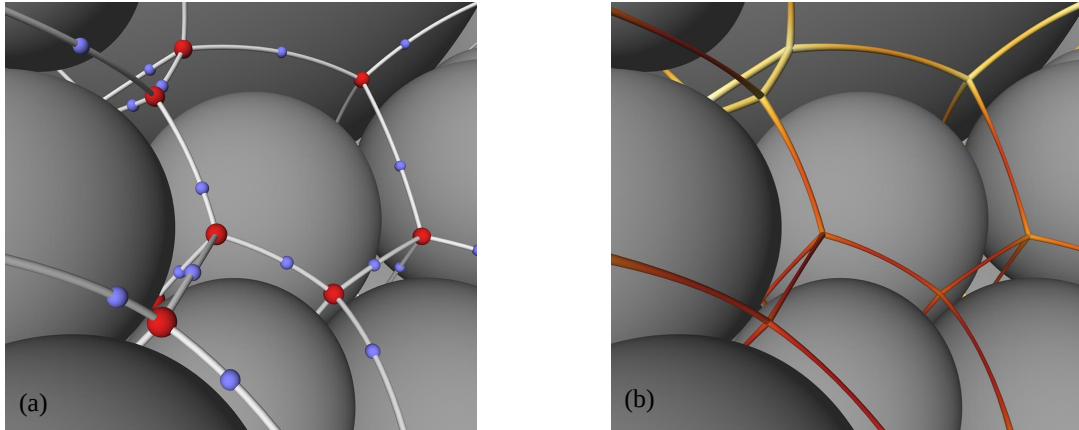
Figure 2: Detail of a Voronoï graph (GGD); (a): red (larger) spheres at crossing indicate the centers of pores, while the blue (smaller) spheres represent the centers of constrictions on the edges; (b): The diameter is color-coded along the edges with yellow (large) to red (small) (color figure online)
