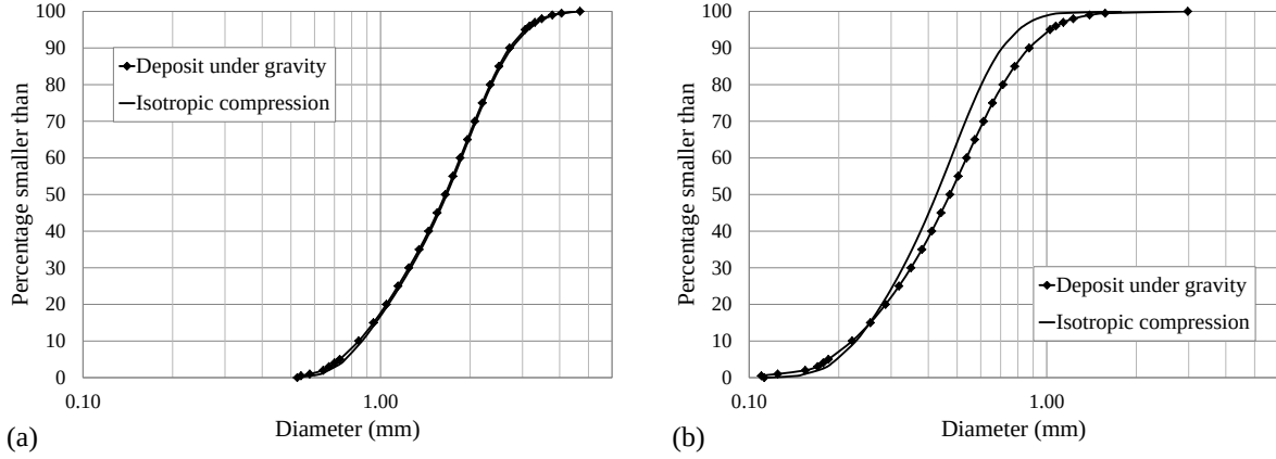
Fig. III.2. CSDs obtained from samples prepared by different techniques (deposit under gravity, isotropic compression); (a): UGL, (b): WG1L
