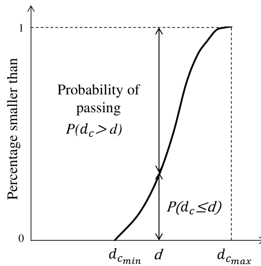
Fig. I.5. Constriction size distribution (CSD) and probability for a fine particle of diameter d to pass a constriction of its own size
