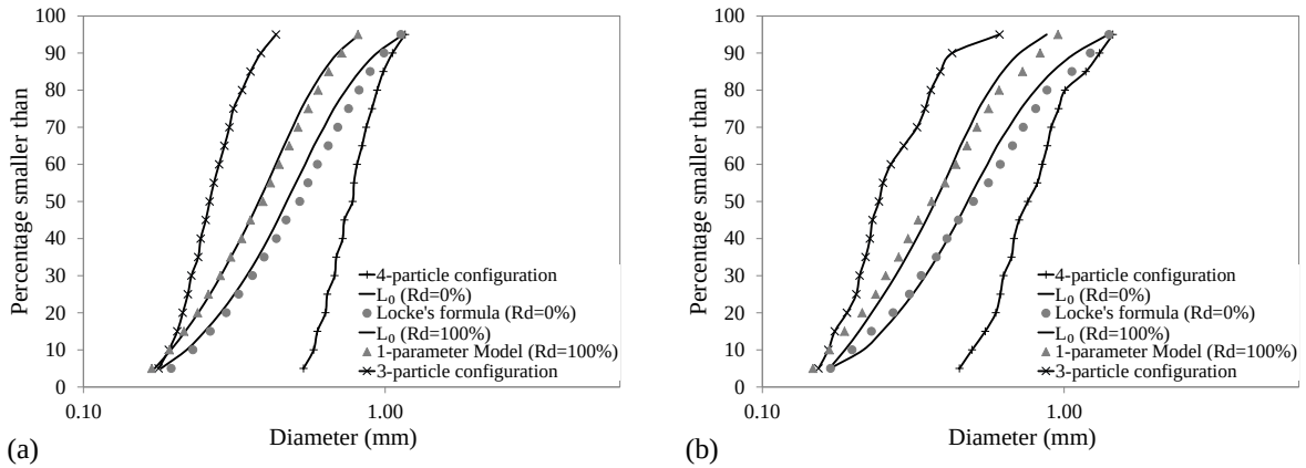
Fig. III.16. Comparison of the CSDs calculated with the analytical method and the Delaunay method ( L_0 computation) for (a): WG2; (b): GG2
